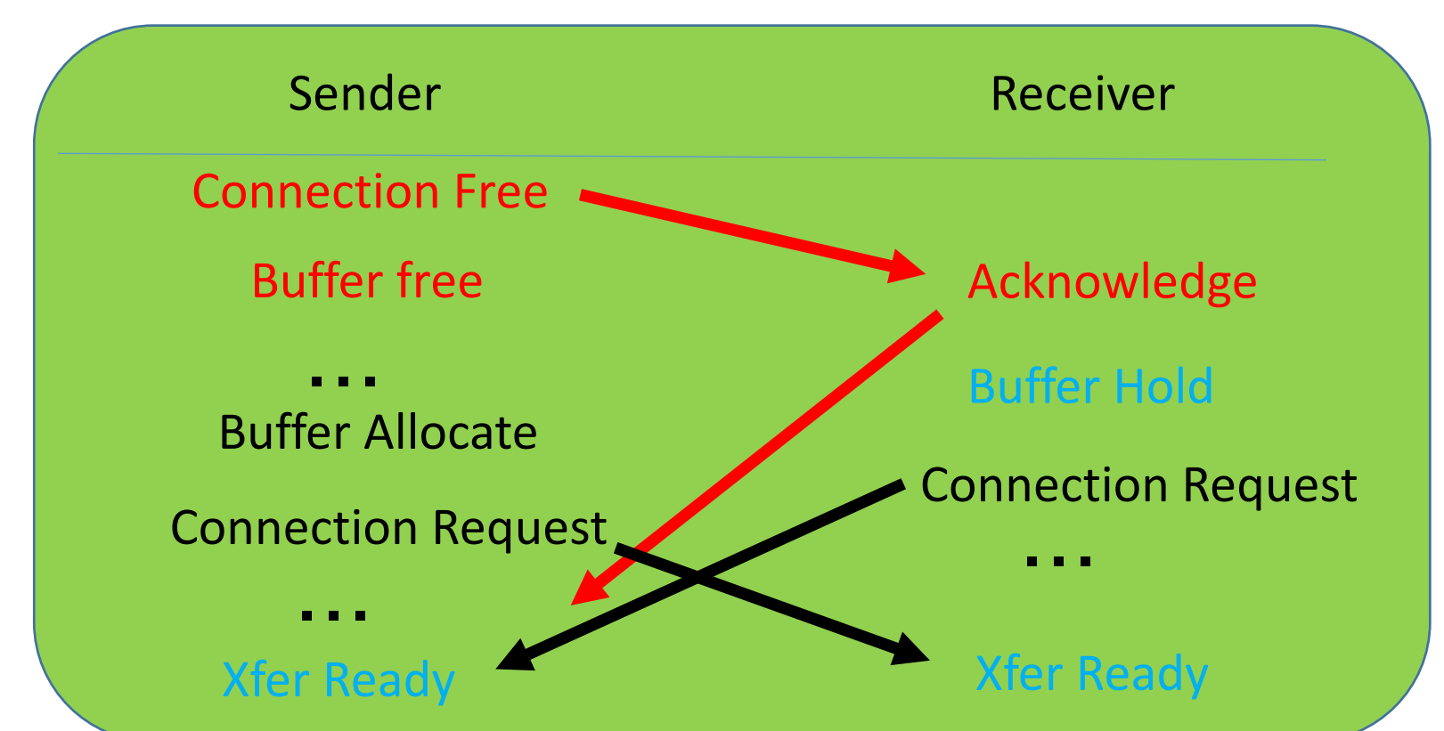
Asynchronous connection and free protocol Red line : Free protocol Black line : Connection protocol
